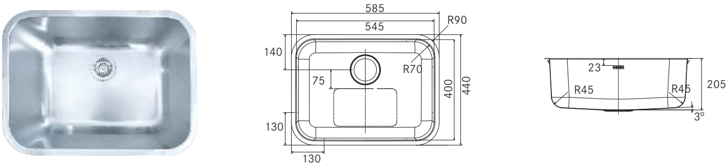
RSX 210-55 (23"x18")
